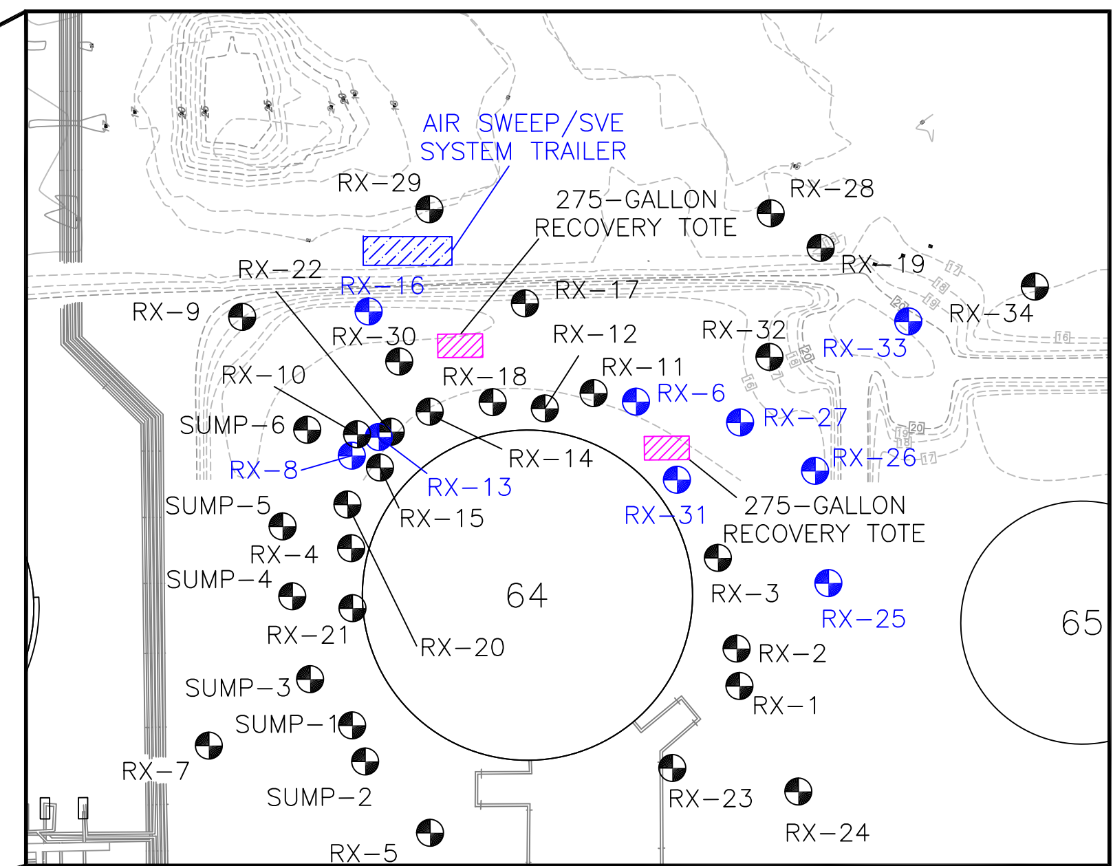
TANK 64 DETAIL
